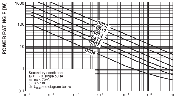
PULSE RATING P \rightarrow 0
