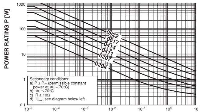
PULSE RATING P \leq P70
